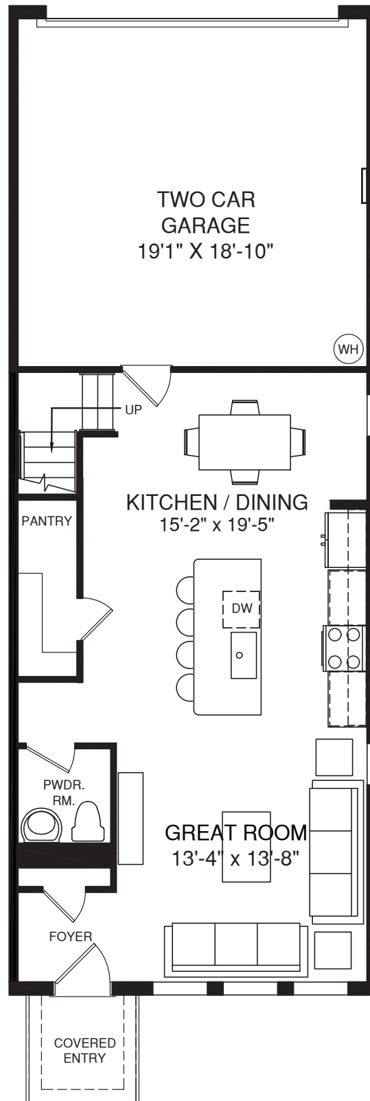
MAIN LEVEL
